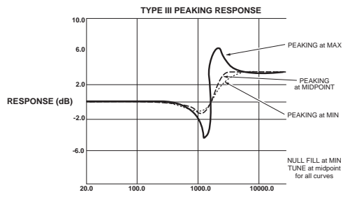
Peaking control
