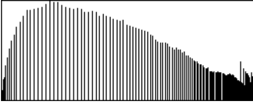
Example of a histogram with gaps
