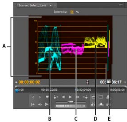
YCbCr Parade scope
