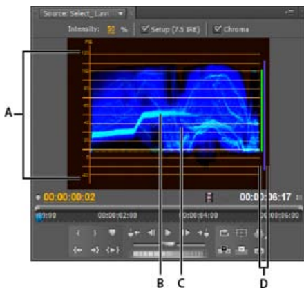
YC Waveform with the chroma control enabled
